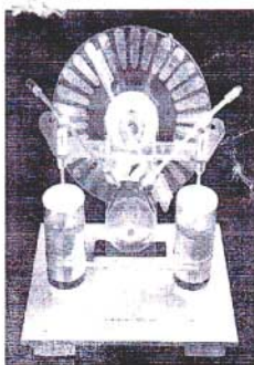
Wimshurst Machine
