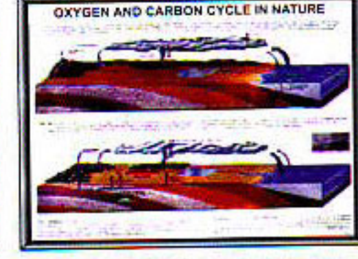
RR080 OXYGEN AND CARBON CYCLE IN NATURE Showing in detail the oxygen & carbon dioxide in the air, photosynthesis and respiration
