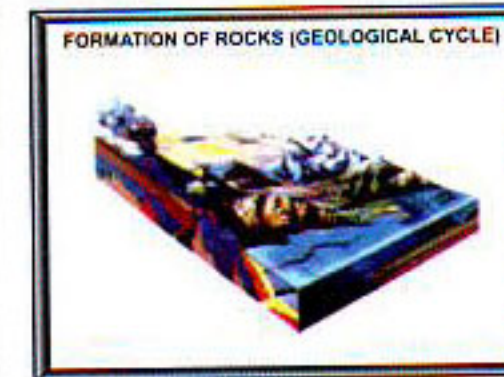
RR082 FORMATION OF ROCKS Show the Geological cycle and the process of ever changing contents of the earth which results in formation of rocks.
