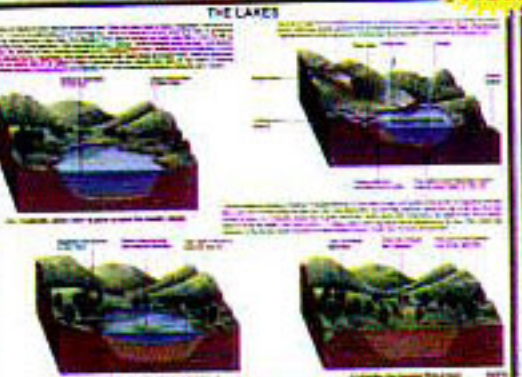
RR088 MODEL OF THE LAKES Shows different kinds of lakes and how lakes become firm ground
