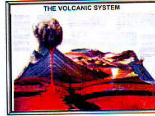
RR079 THE VOLCANIC SYSTEM Shows different parameters how volcanoes take place as the hanging feature there after.
